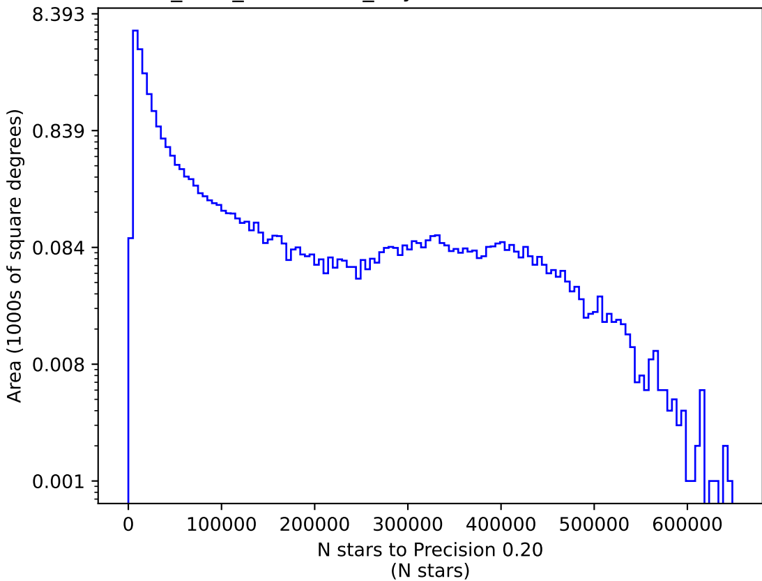
start_date_do270v3.4_10yrs z: N stars to Precision 0.20
