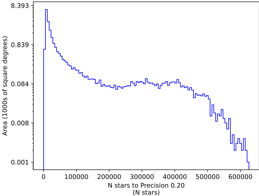
start_date_do270v3.4_10yrs y: N stars to Precision 0.20
