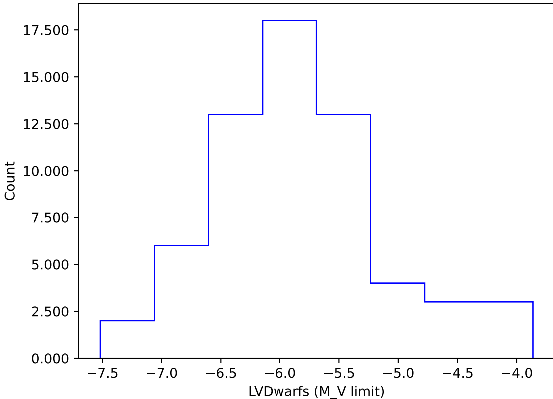
start_date_do270v3.4_10yrs gi: LVDwarfs
