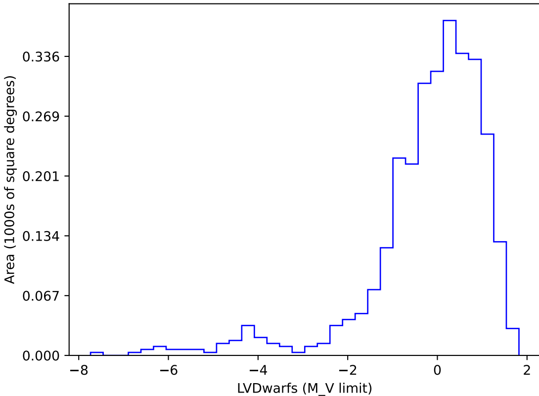
start_date_do270v3.4_10yrs gi SCP: LVDwarfs
