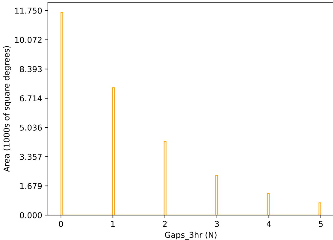
start_date_do270v3.4_10yrs r band: Gaps_3hr
