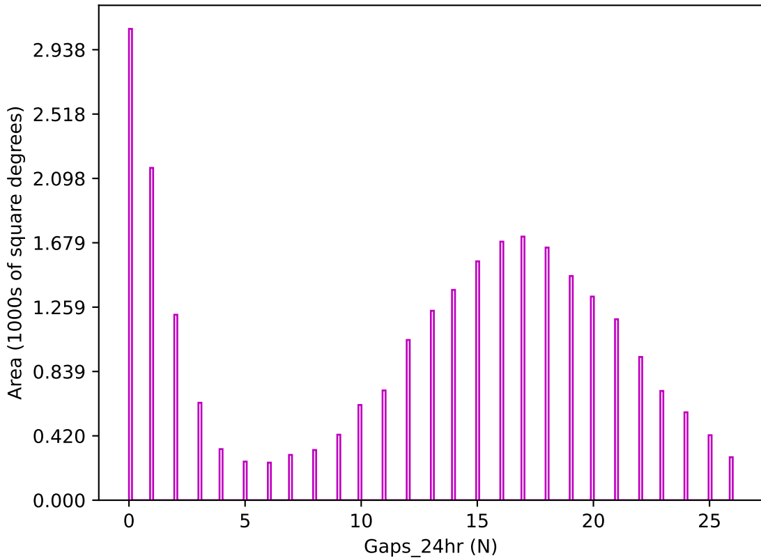
start_date_do270v3.4_10yrs z band: Gaps_24hr
