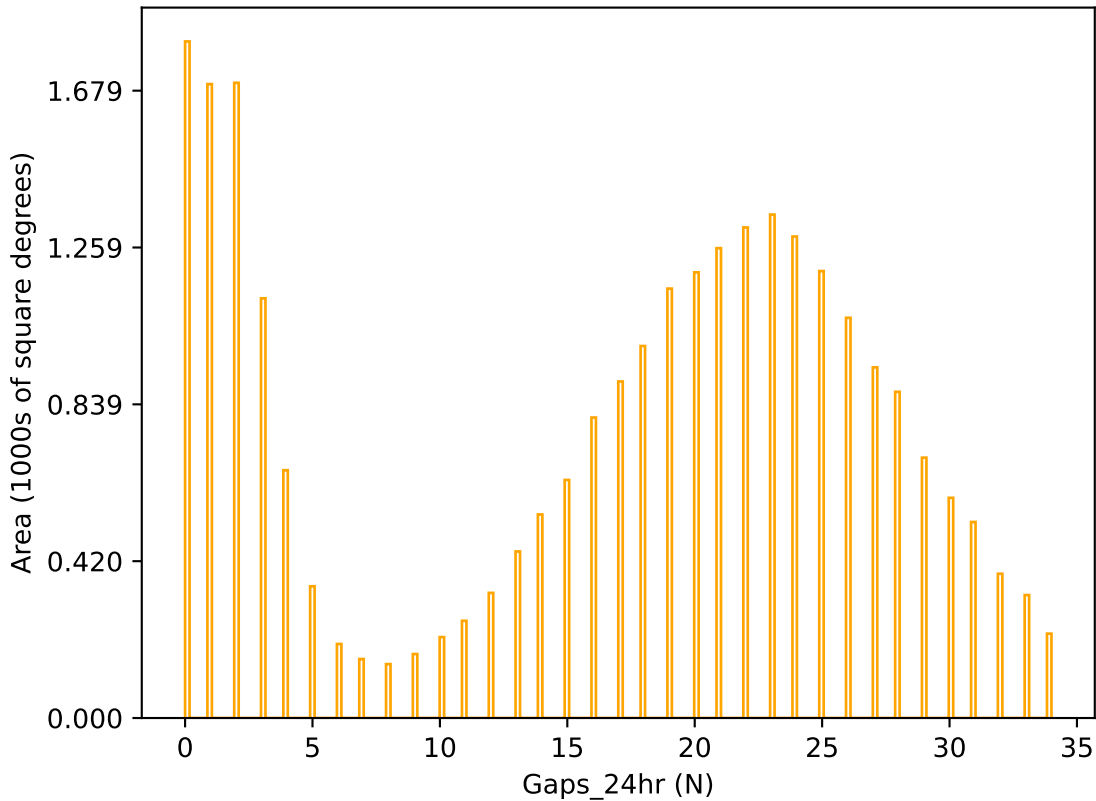
start_date_do270v3.4_10yrs r band: Gaps_24hr
