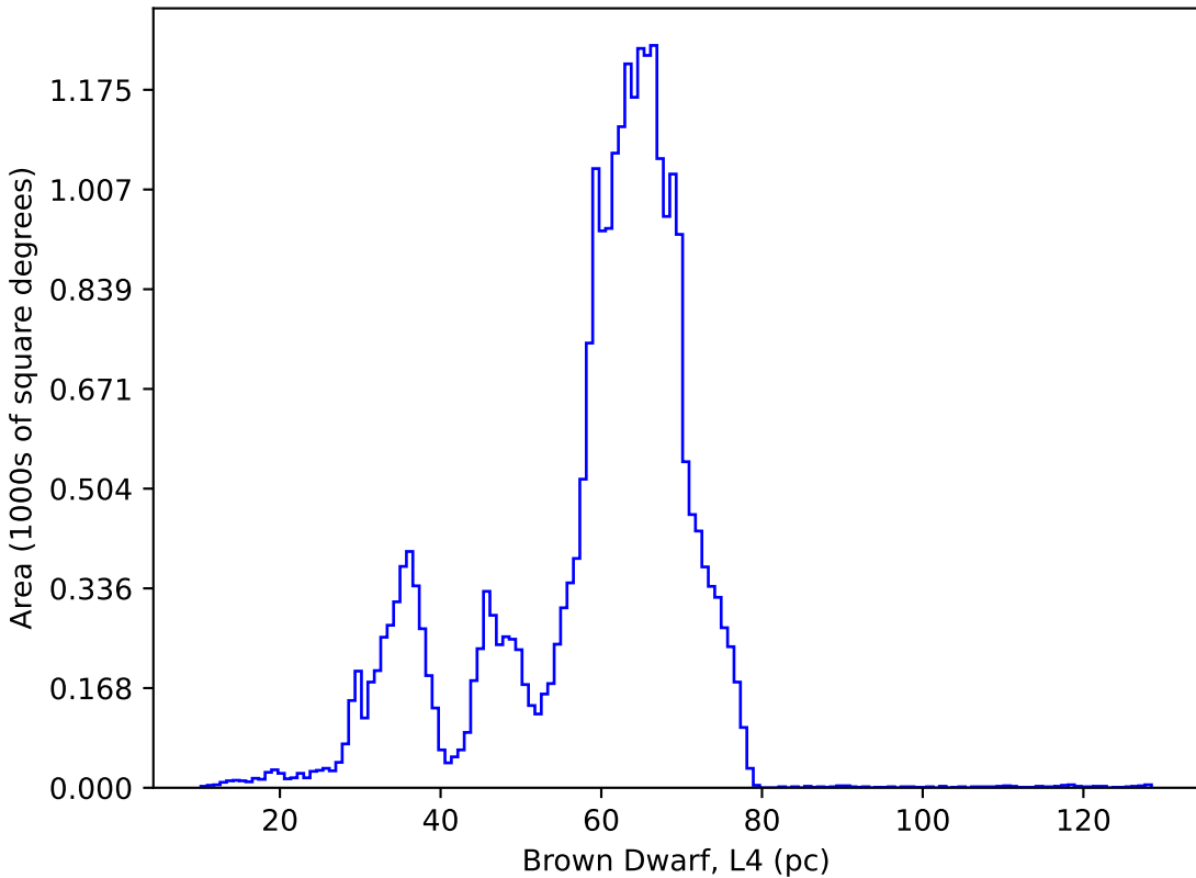
start_date_do270v3.4_10yrs : Brown Dwarf, L4
