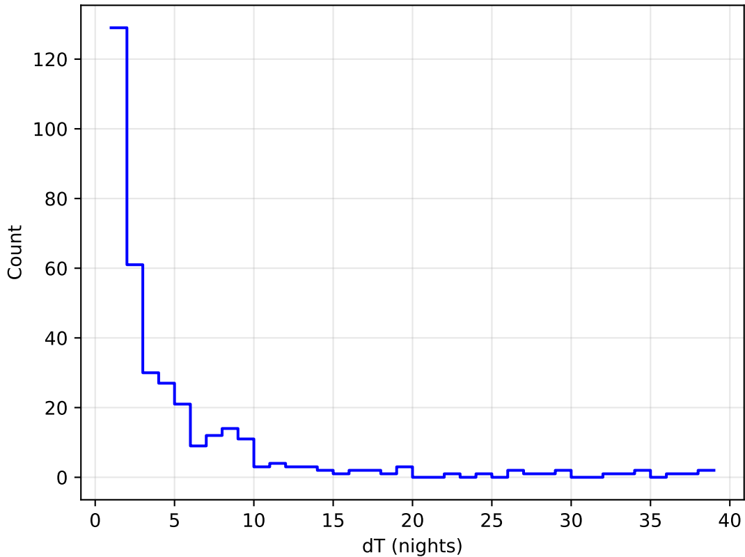
start_date_do270v3.4_10yrs all bands: DD:WFD Delta Nights Histogram
