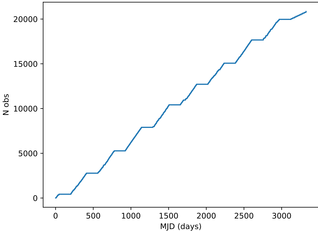
start_date_do270v3.4_10yrs all bands: DD:EDFS Cumulative NVisits
