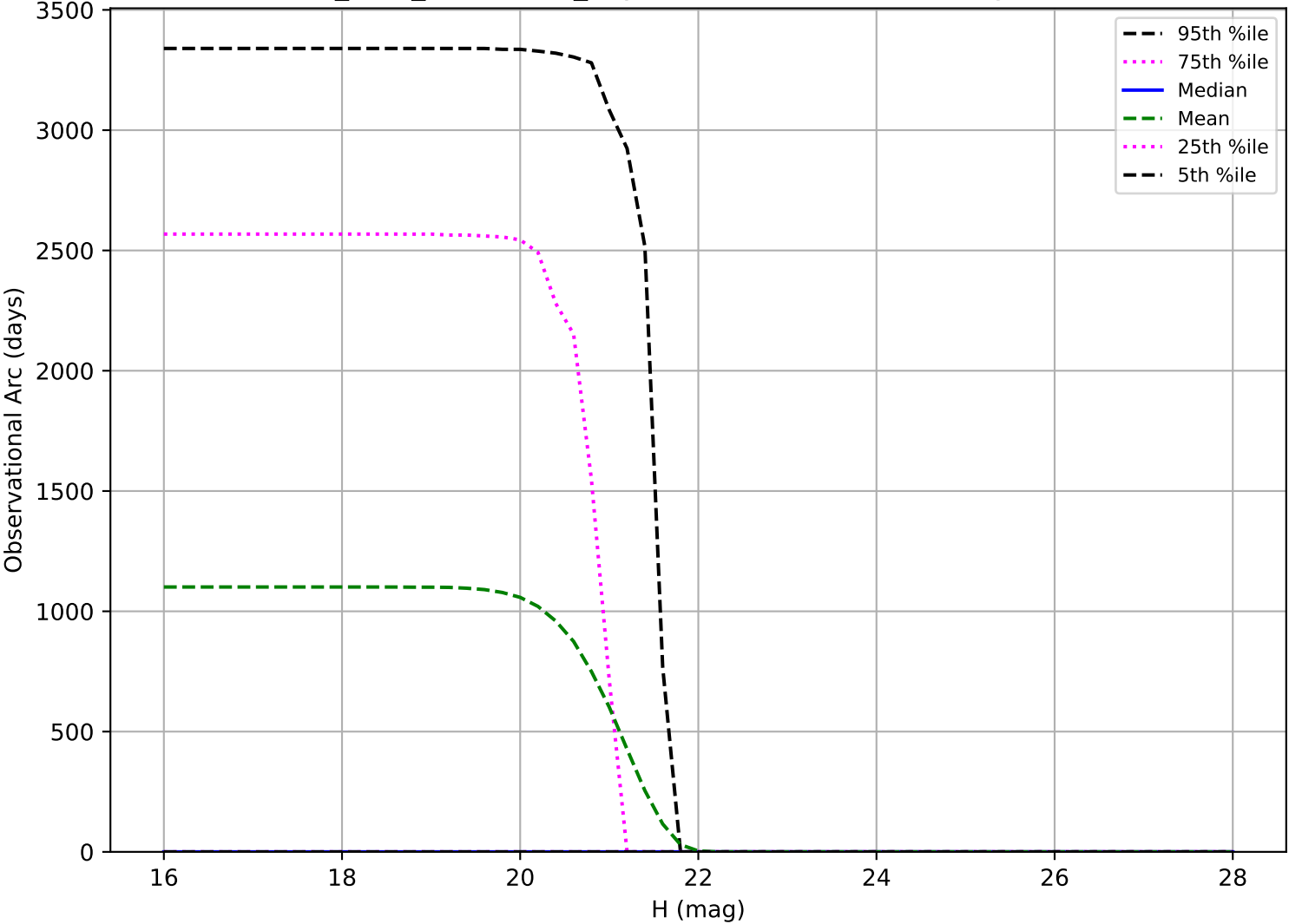
start_date_do180v3.4_10yrs: Observational Arc Length Vatira
