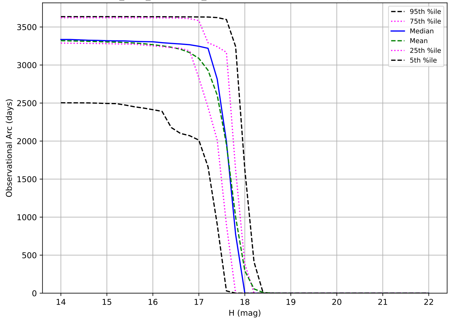
start_date_do180v3.4_10yrs: Observational Arc Length Trojan
