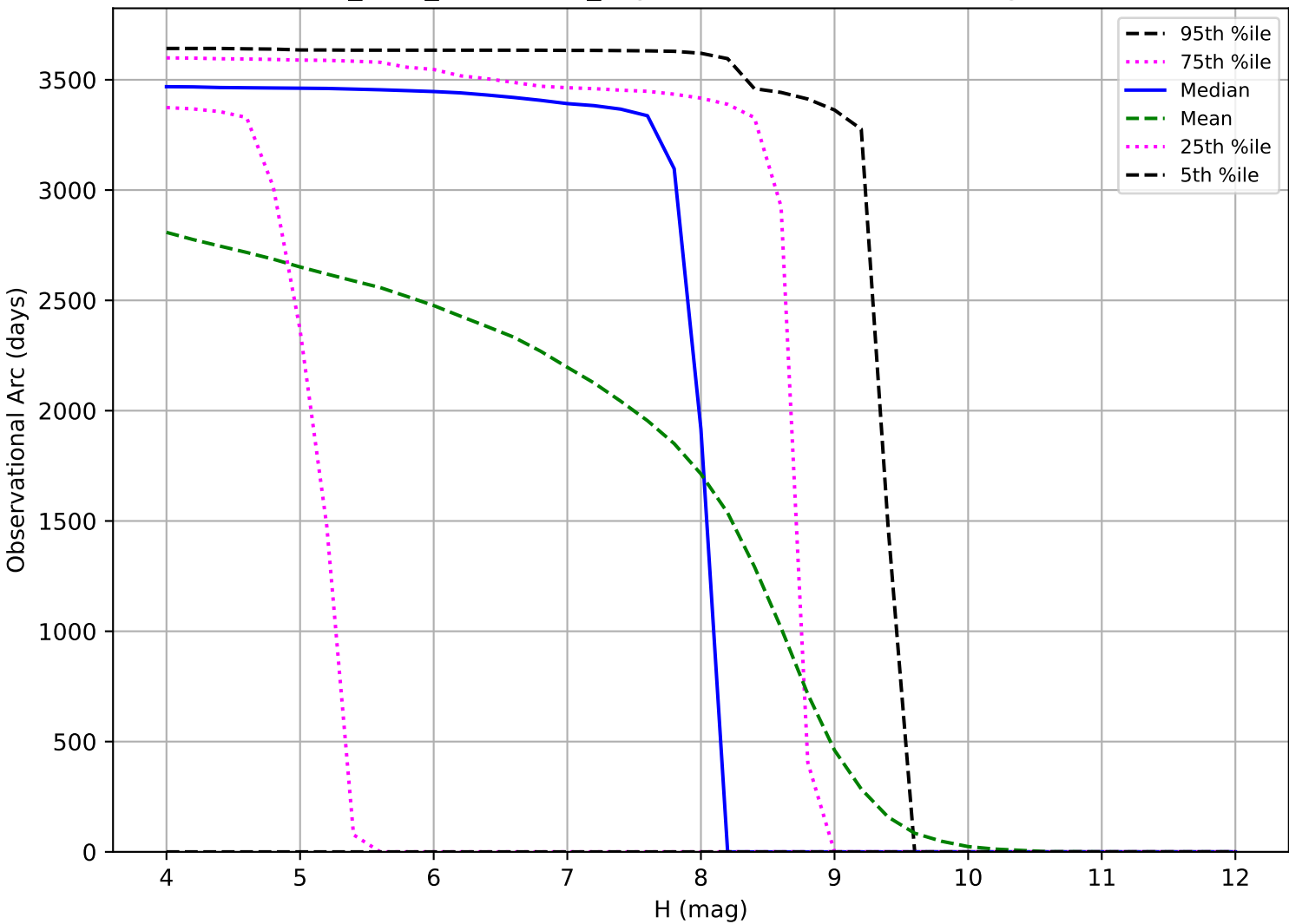
start_date_do180v3.4_10yrs: Observational Arc Length TNO
