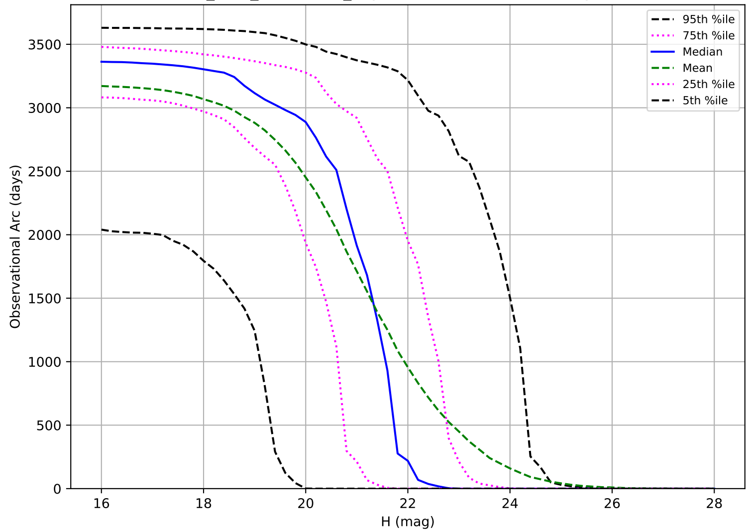
start_date_do180v3.4_10yrs: Observational Arc Length PHA
