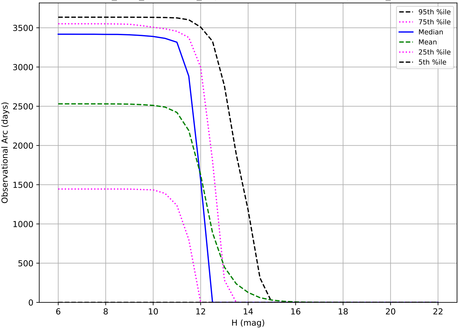
start_date_do180v3.4_10yrs: Observational Arc Length OCC_r20
