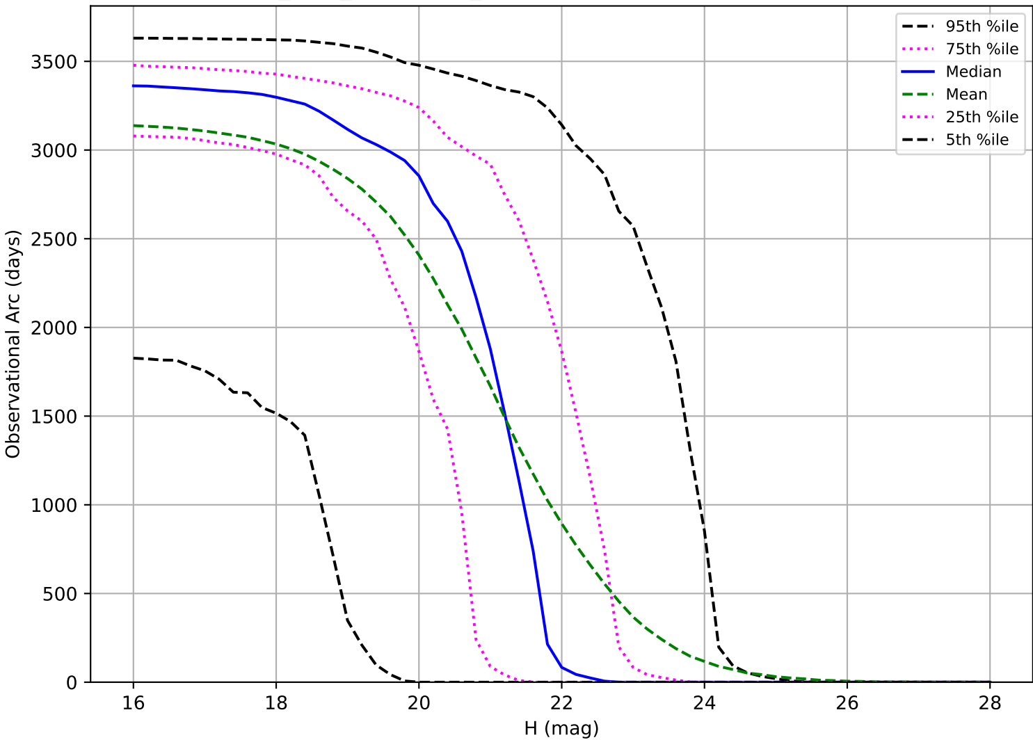
start_date_do180v3.4_10yrs: Observational Arc Length NEO
