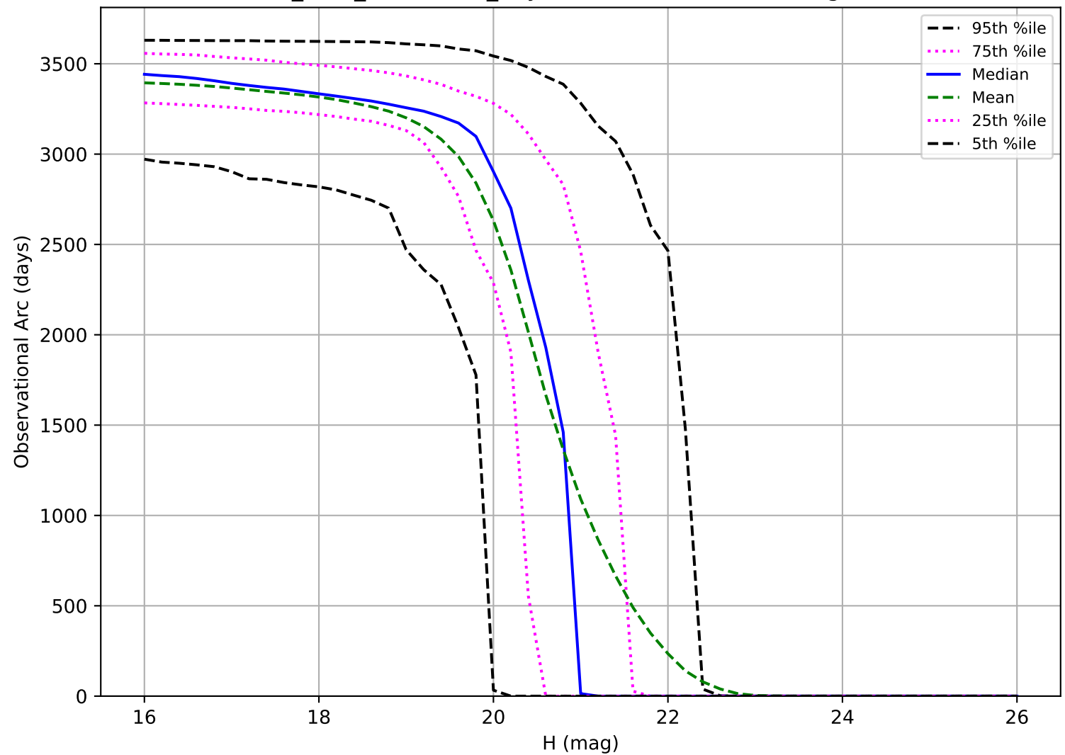
start_date_do180v3.4_10yrs: Observational Arc Length MBA
