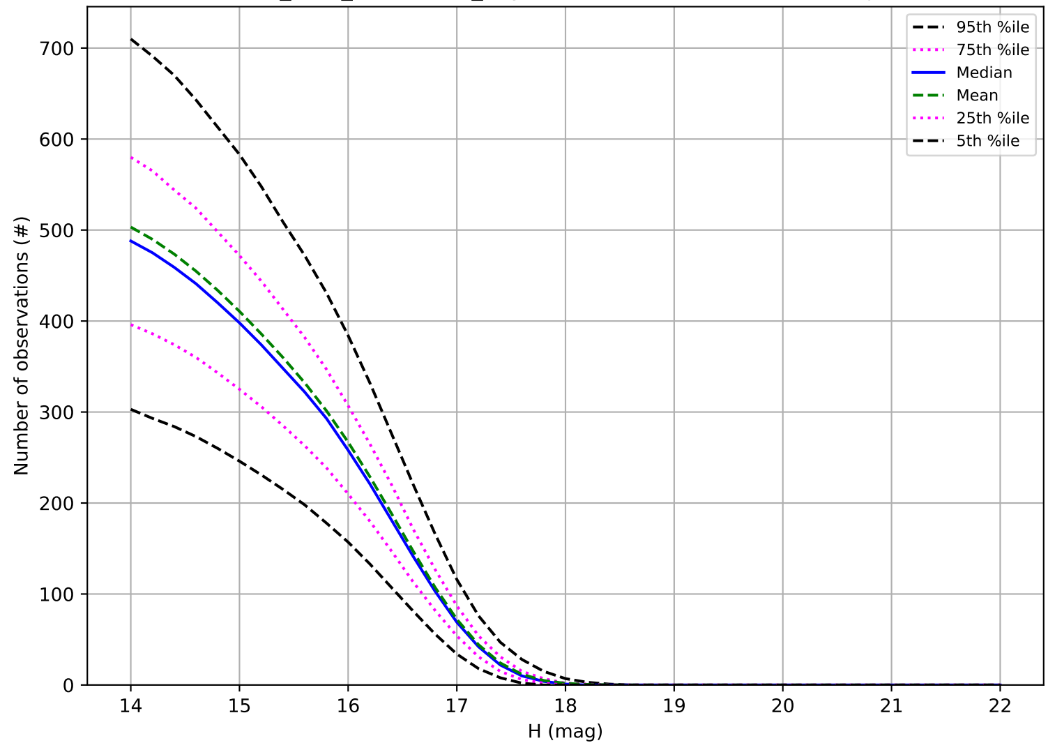
start_date_do180v3.4_10yrs: Number of observations Trojan
