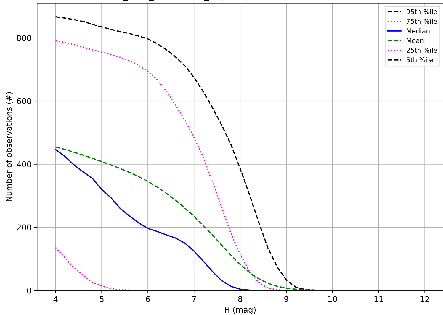
start_date_do180v3.4_10yrs: Number of observations TNO
