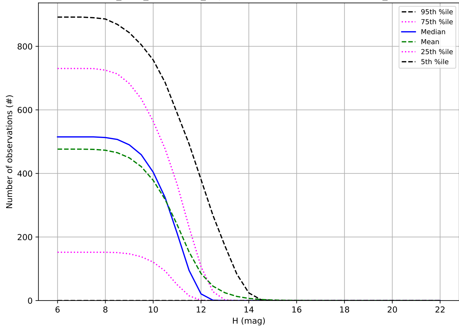
start_date_do180v3.4_10yrs: Number of observations OCC_r20
