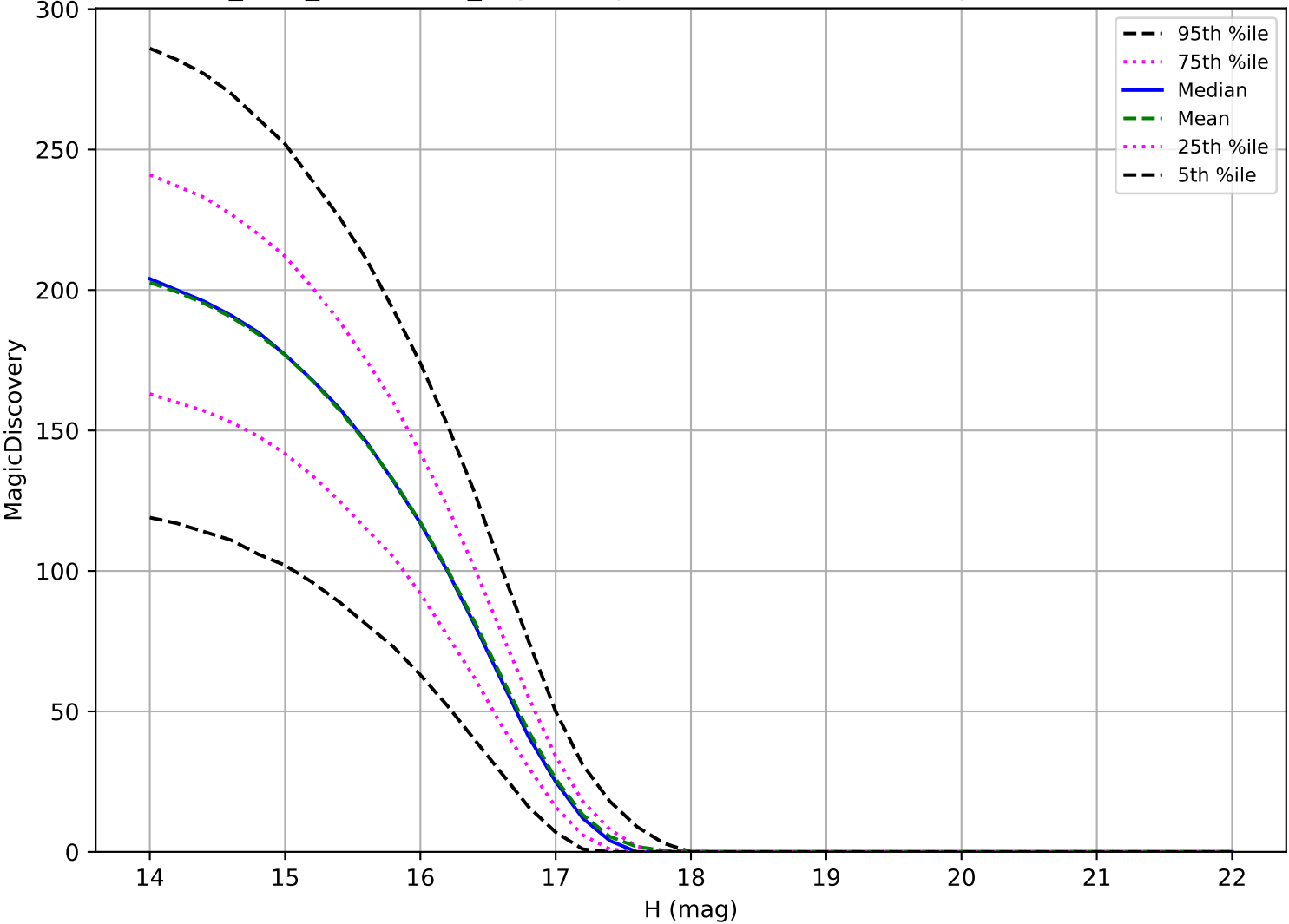
start_date_do180v3.4_10yrs: Trojan 6 detections in 60 nights detection loss
