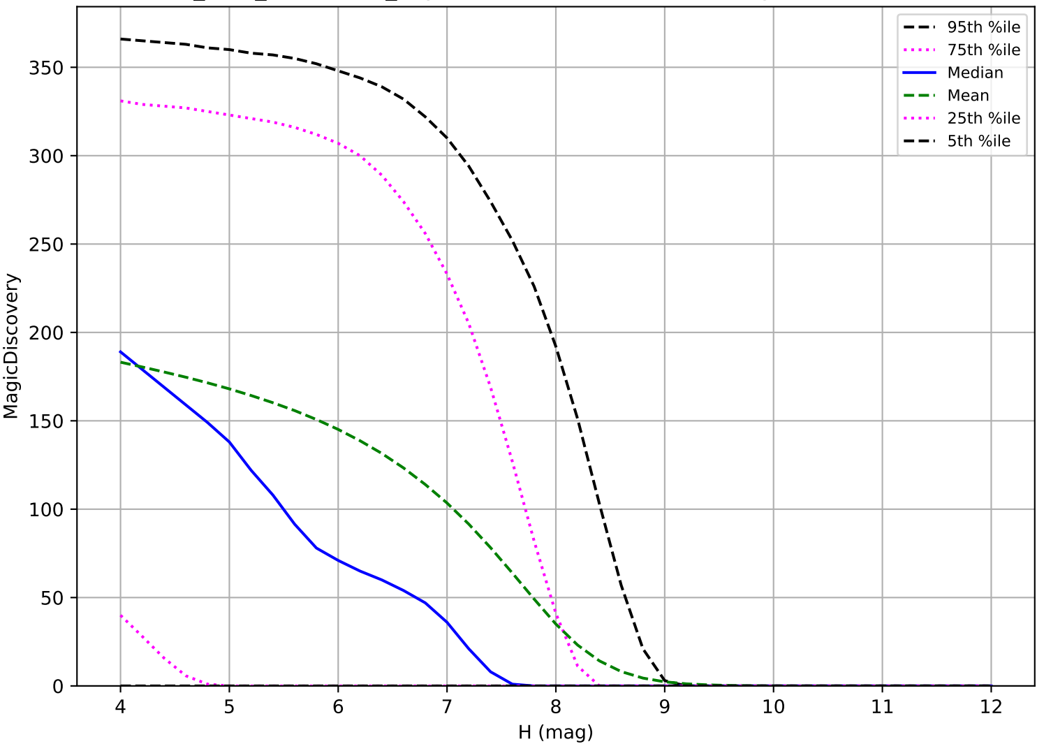
start_date_do180v3.4_10yrs: TNO 6 detections in 60 nights detection loss
