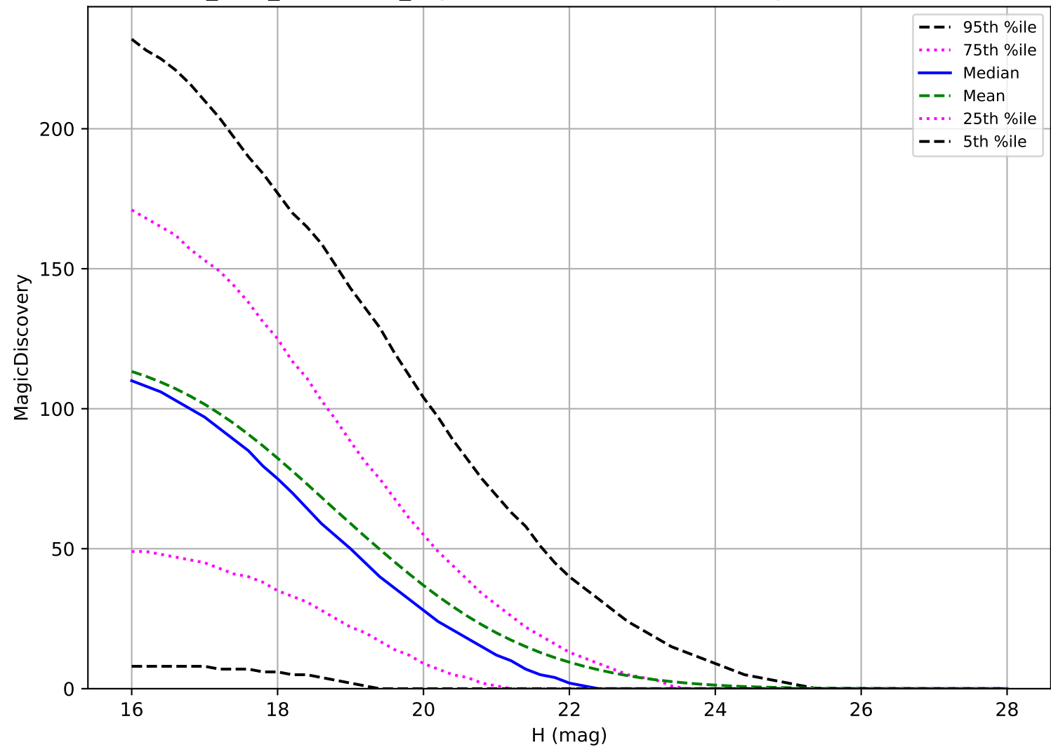
start_date_do180v3.4_10yrs: PHA 6 detections in 60 nights detection loss
