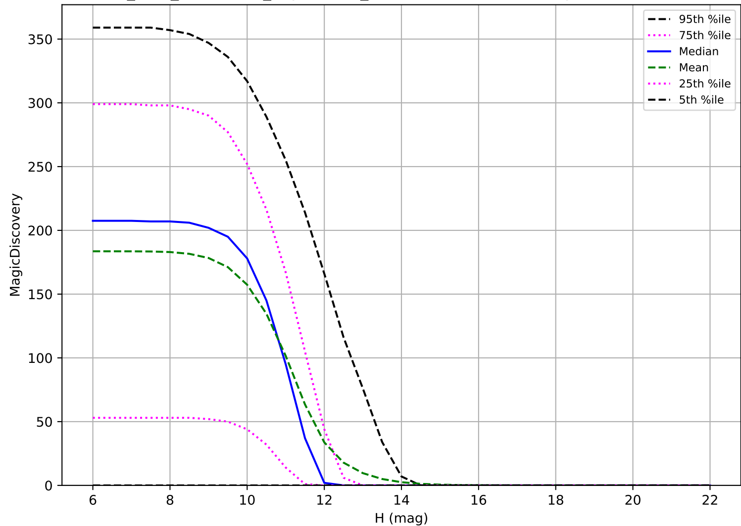
start_date_do180v3.4_10yrs: OCC_r20 6 detections in 60 nights detection loss
