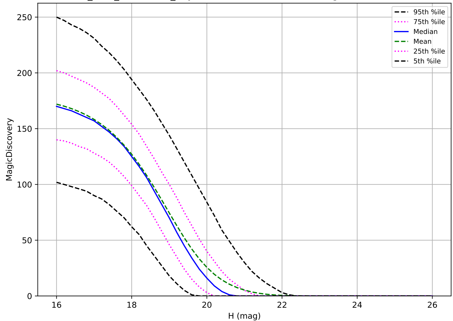
start_date_do180v3.4_10yrs: MBA 6 detections in 60 nights detection loss
