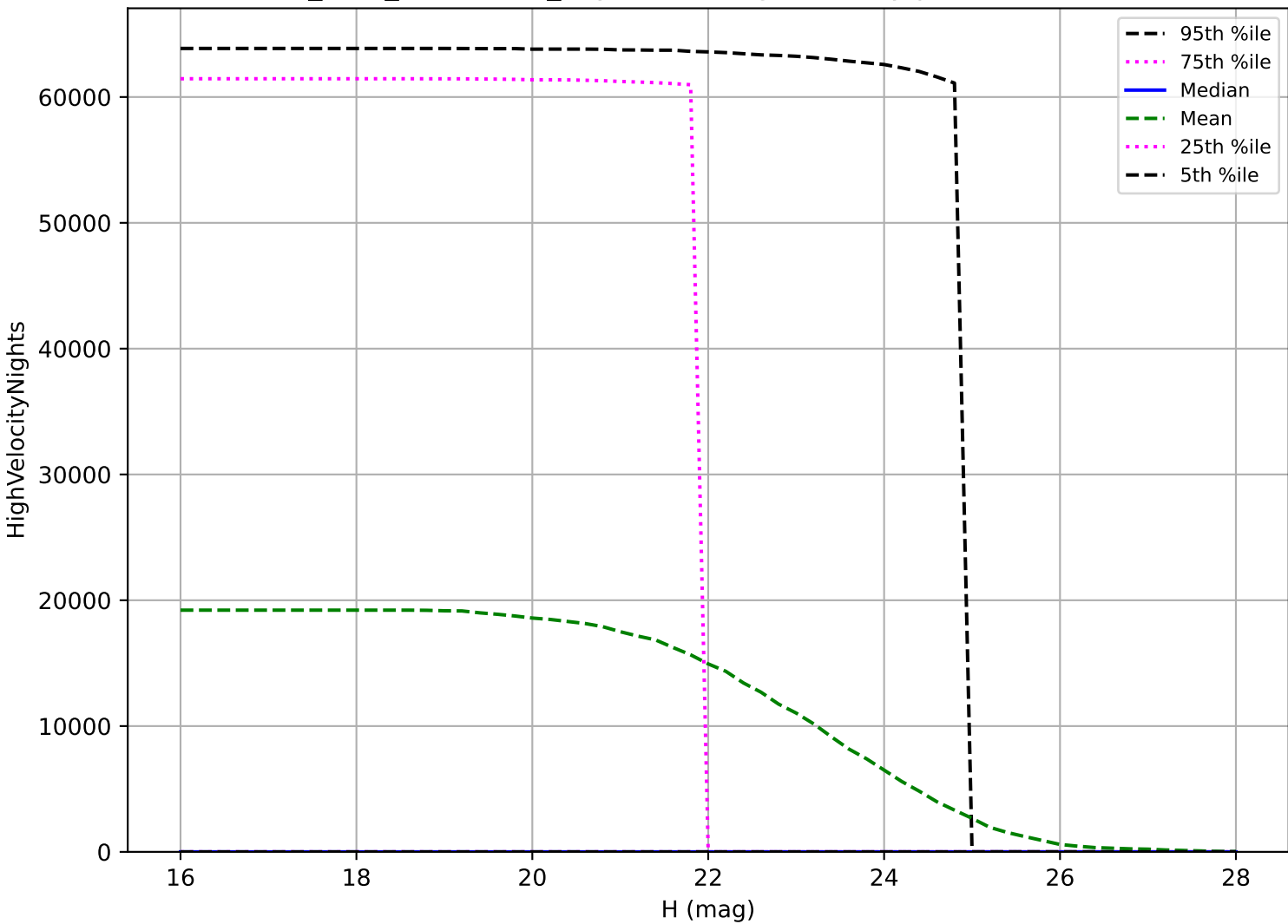
start_date_do180v3.4_10yrs: NEO High velocity pair detection loss
