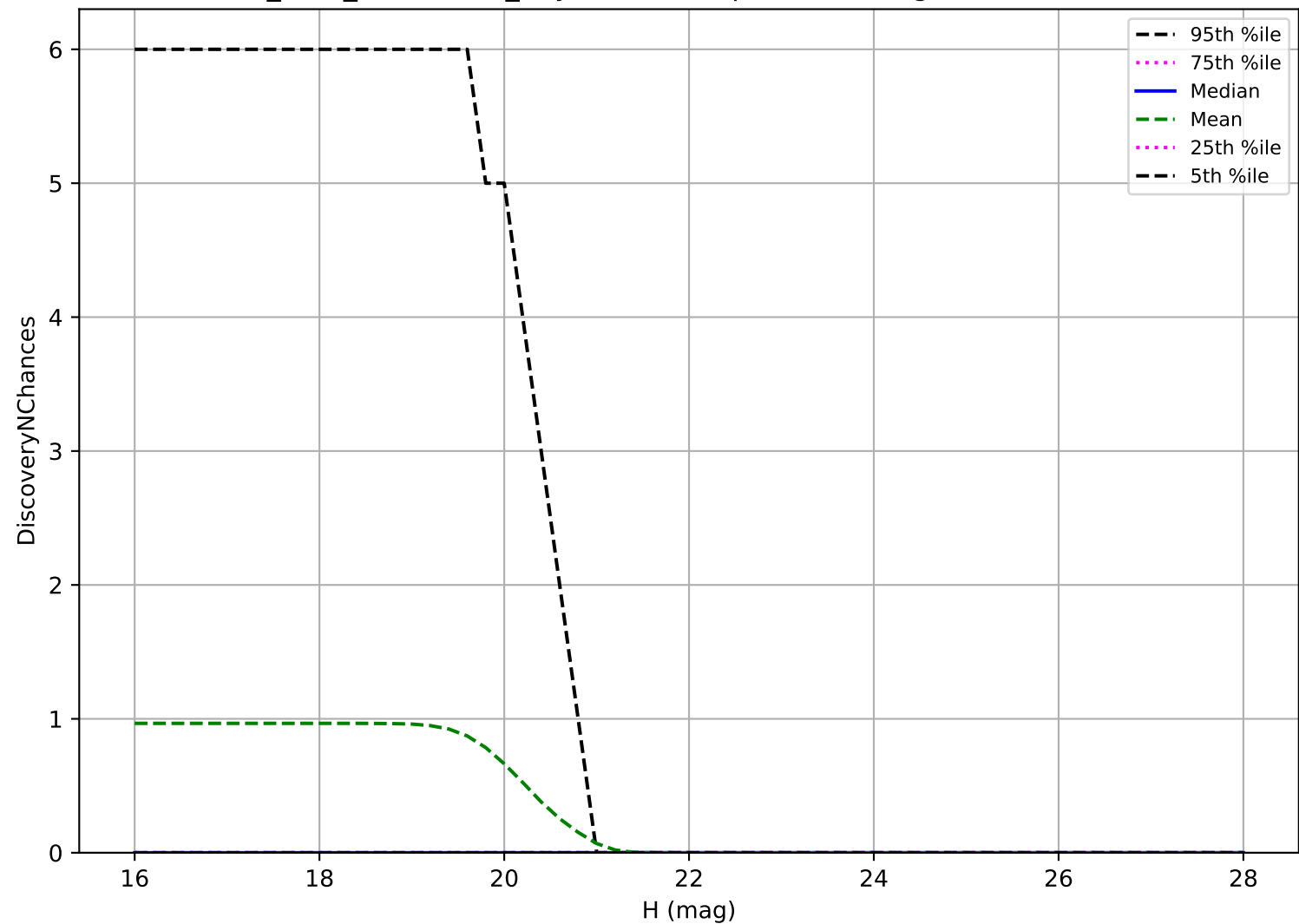
start_date_do180v3.4_10yrs: Vatira 3 pairs in 15 nights detection loss
