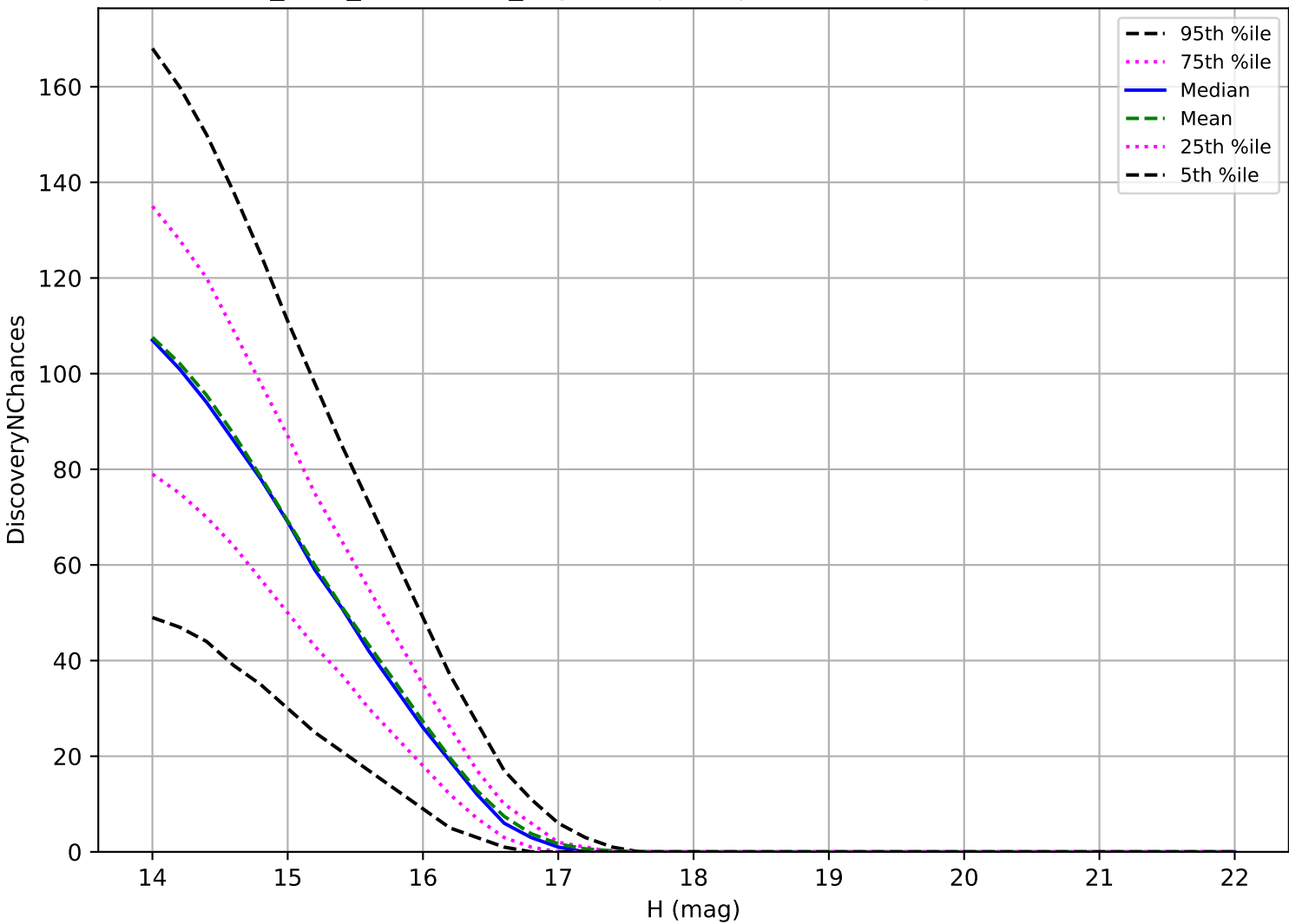
start_date_do180v3.4_10yrs: Trojan 3 pairs in 15 nights detection loss
