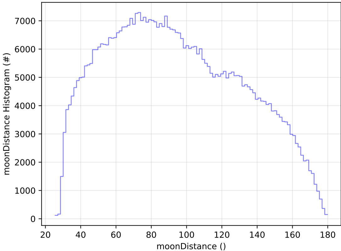
start_date_do180v3.4_10yrs WFD i band: moonDistance Histogram
