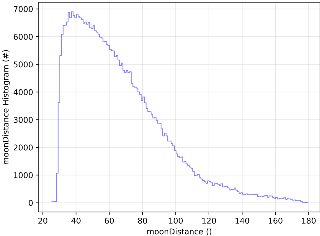
start_date_do180v3.4_10yrs All sky y band: moonDistance Histogram
