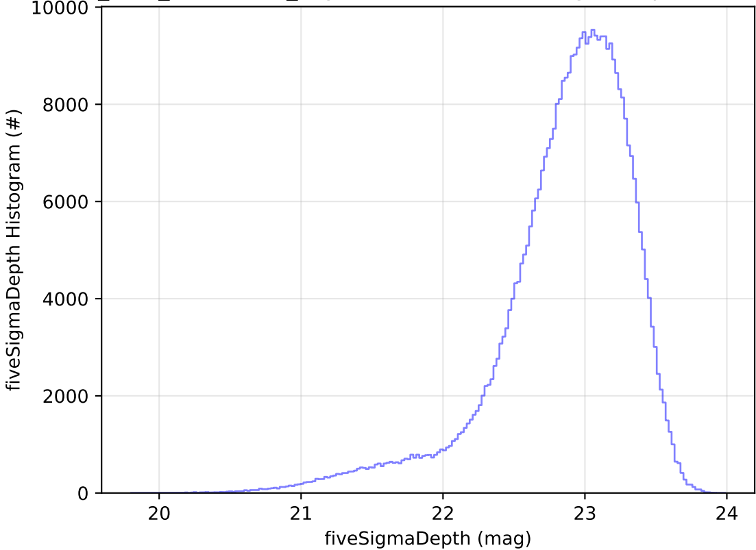
start_date_do180v3.4_10yrs WFD z band: fiveSigmaDepth Histogram
