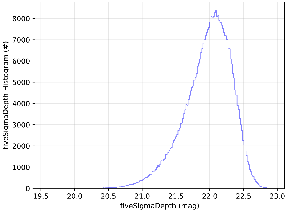
start_date_do180v3.4_10yrs WFD y band: fiveSigmaDepth Histogram
