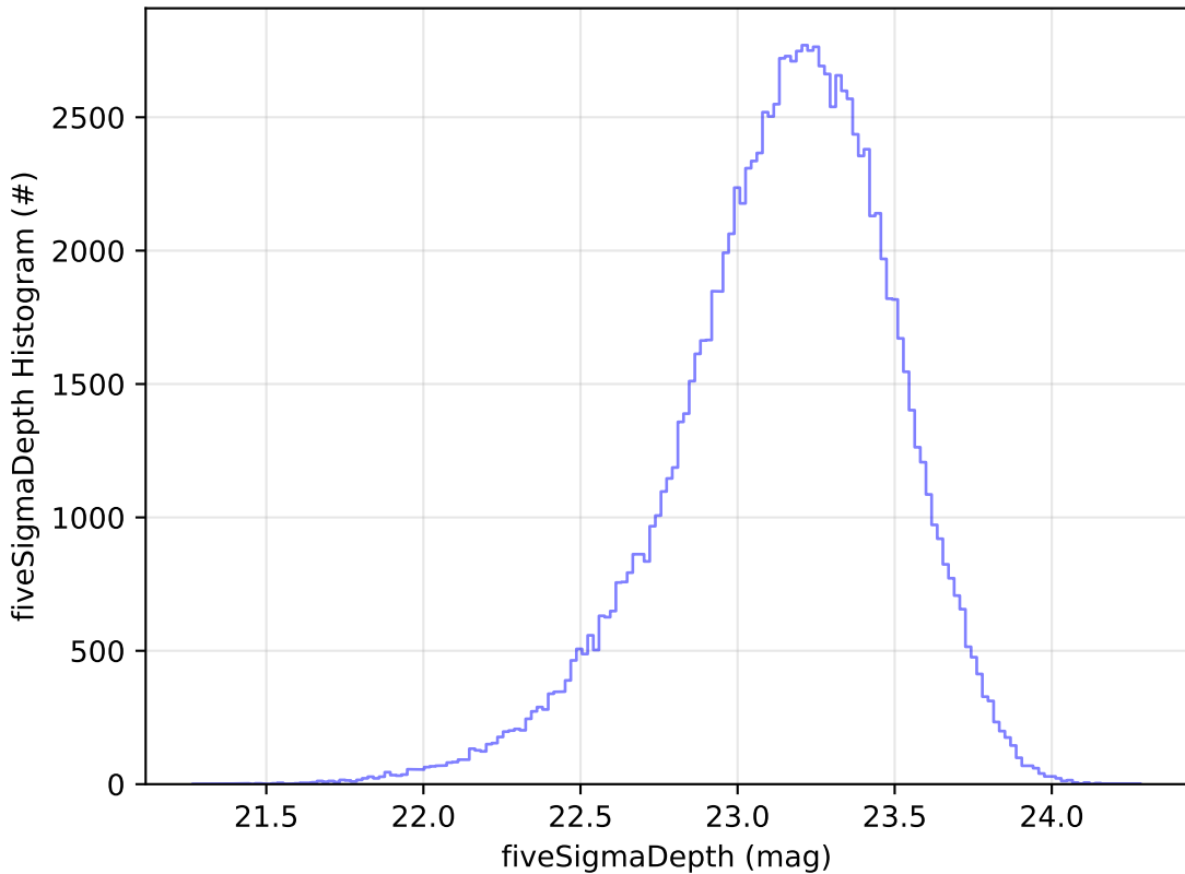
start_date_do180v3.4_10yrs WFD u band: fiveSigmaDepth Histogram
