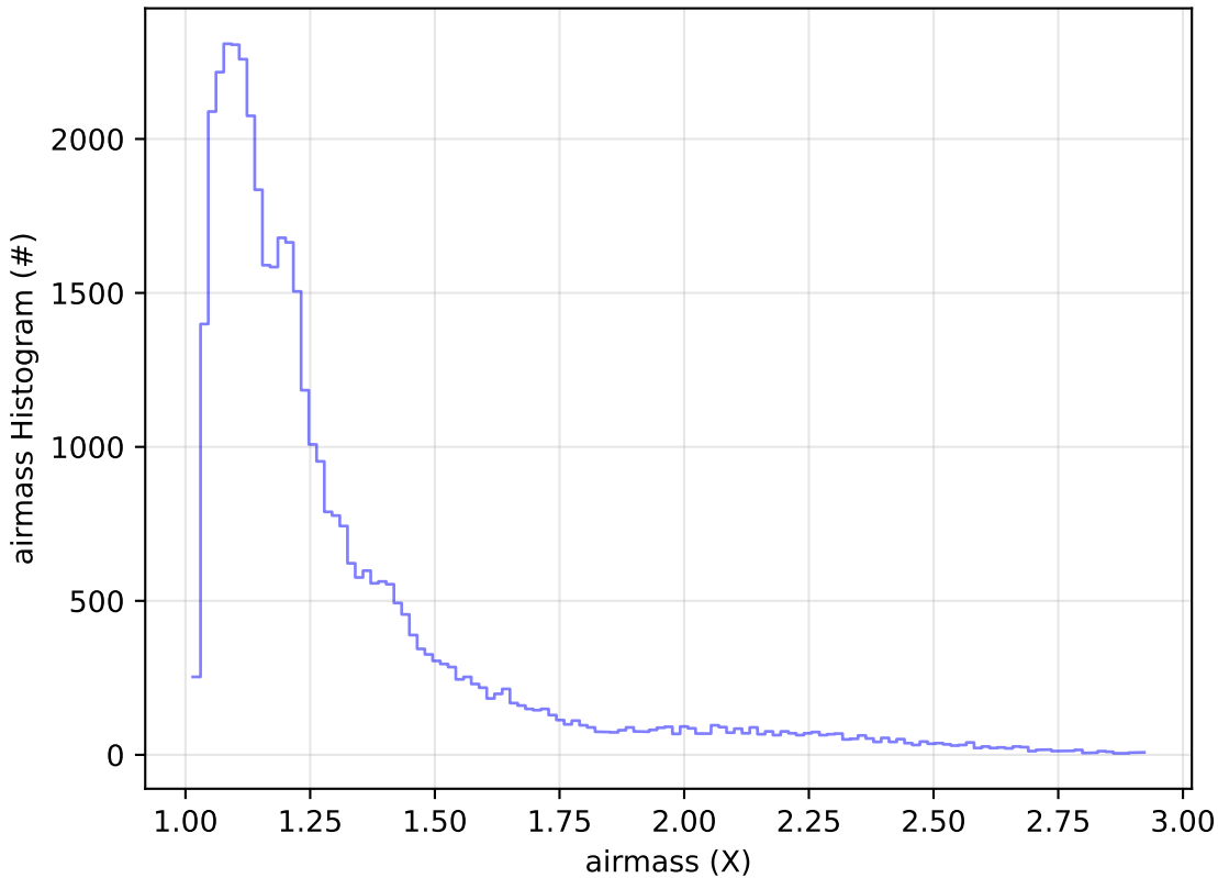
start_date_do180v3.4_10yrs Yr 1 z band: airmass Histogram
