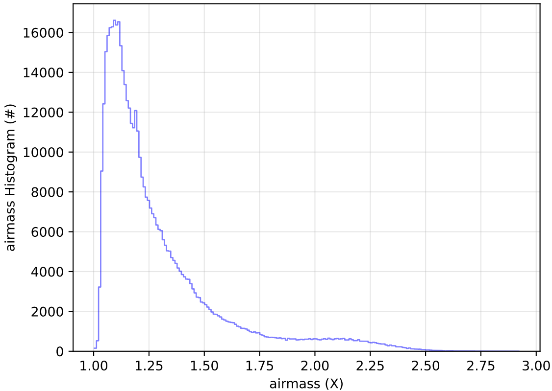
start_date_do180v3.4_10yrs All sky r band: airmass Histogram
