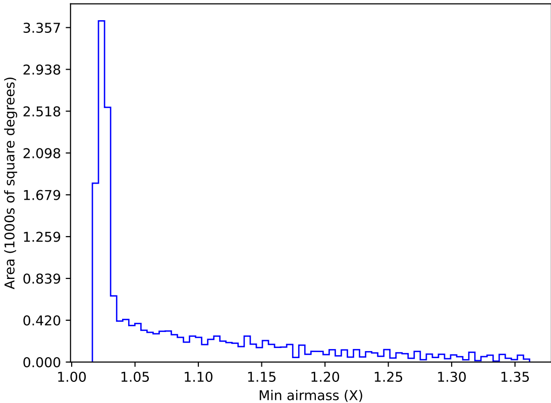
start_date_do180v3.4_10yrs WFD all bands: Min airmass
