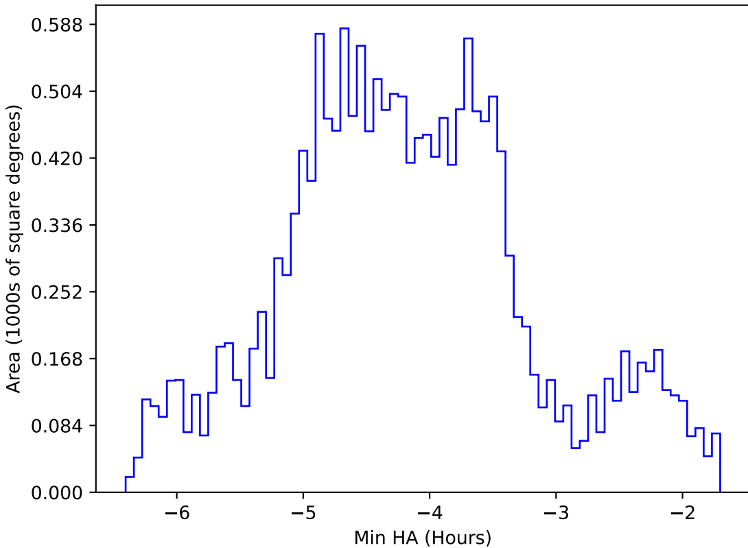
start_date_do180v3.4_10yrs WFD g band: Min HA
