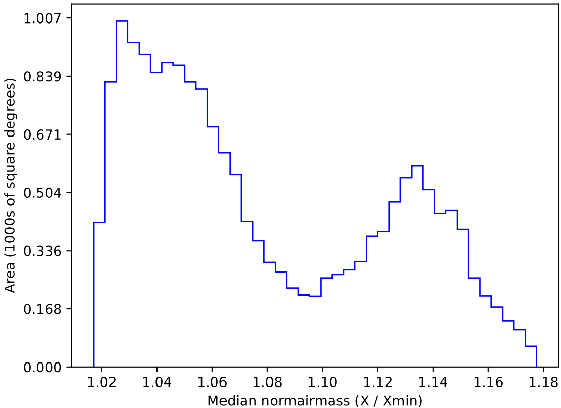
start_date_do180v3.4_10yrs WFD i band: Median normairmass
