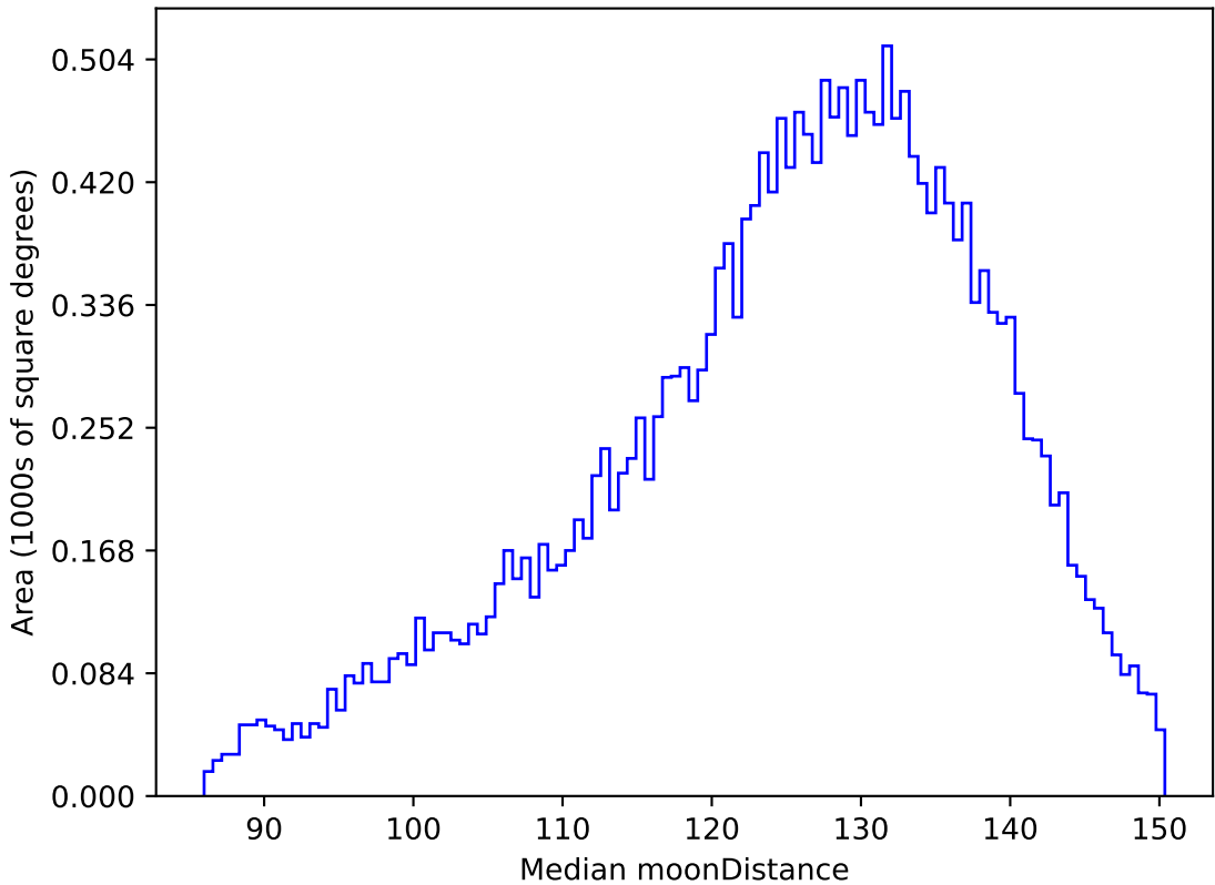
start_date_do180v3.4_10yrs All sky u band: Median moonDistance
