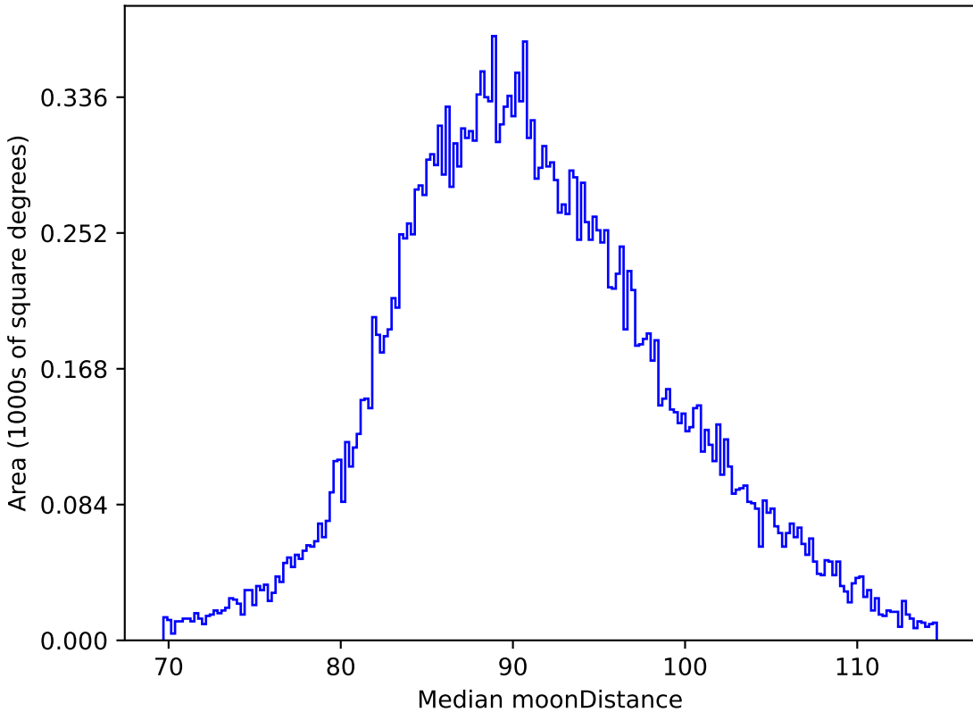
start_date_do180v3.4_10yrs All sky i band: Median moonDistance
