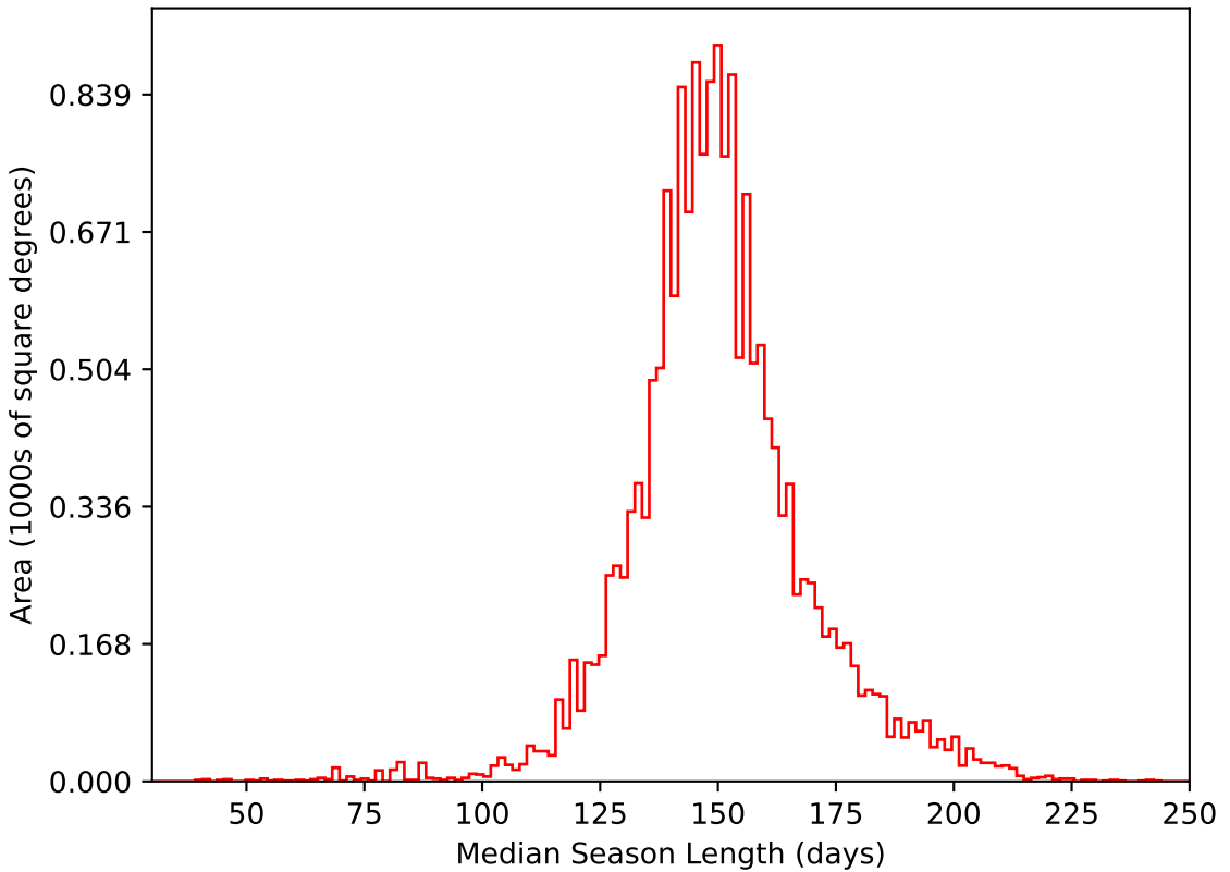
start_date_do180v3.4_10yrs WFD i band: Median Season Length
