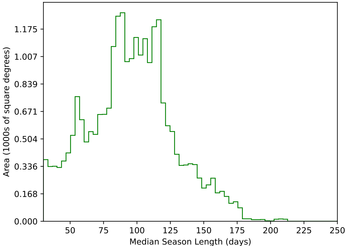
start_date_do180v3.4_10yrs All sky g band: Median Season Length
