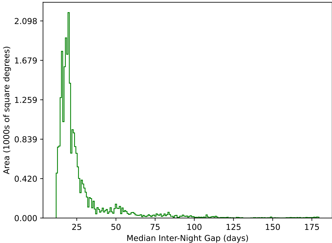
start_date_do180v3.4_10yrs All sky g band: Median Inter-Night Gap
