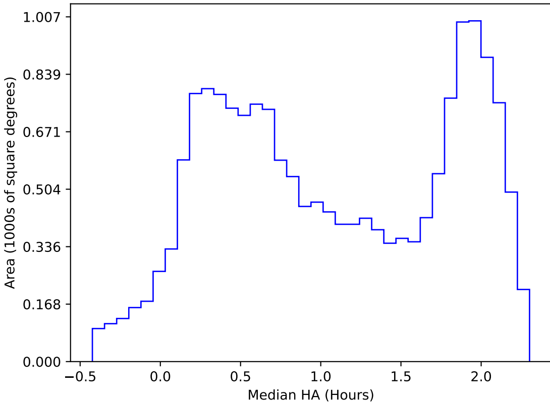
start_date_do180v3.4_10yrs WFD i band: Median HA
