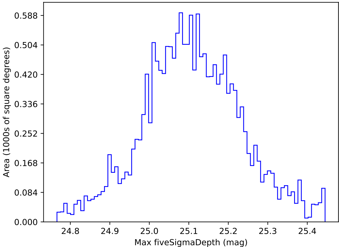
start_date_do180v3.4_10yrs WFD g band: Max fiveSigmaDepth
