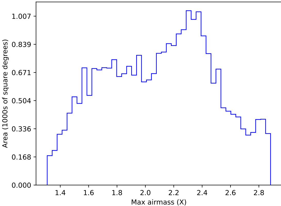
start_date_do180v3.4_10yrs Yr 1 all bands: Max airmass
