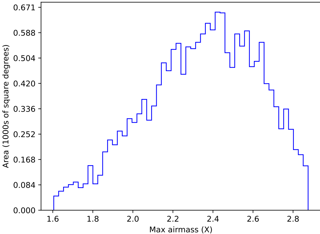
start_date_do180v3.4_10yrs WFD y band: Max airmass
