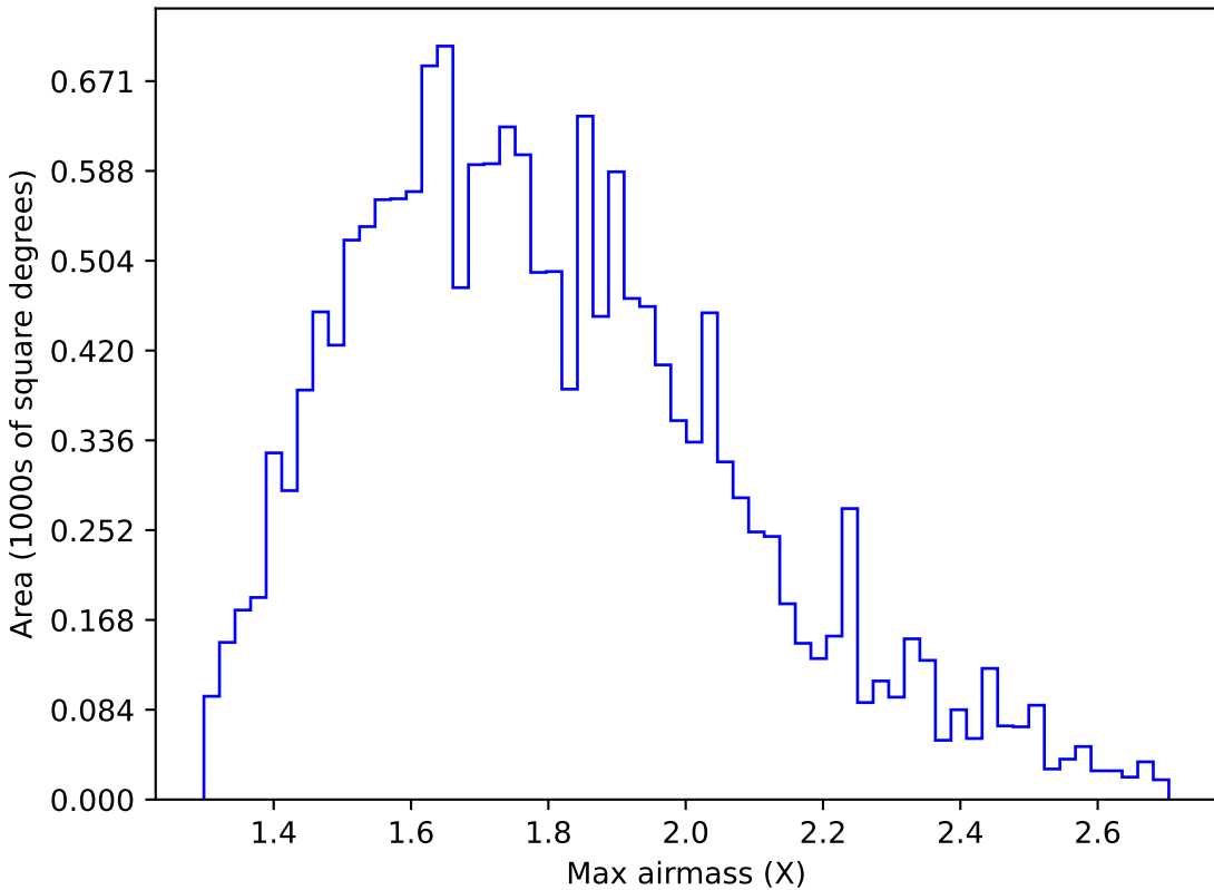
start_date_do180v3.4_10yrs WFD u band: Max airmass
