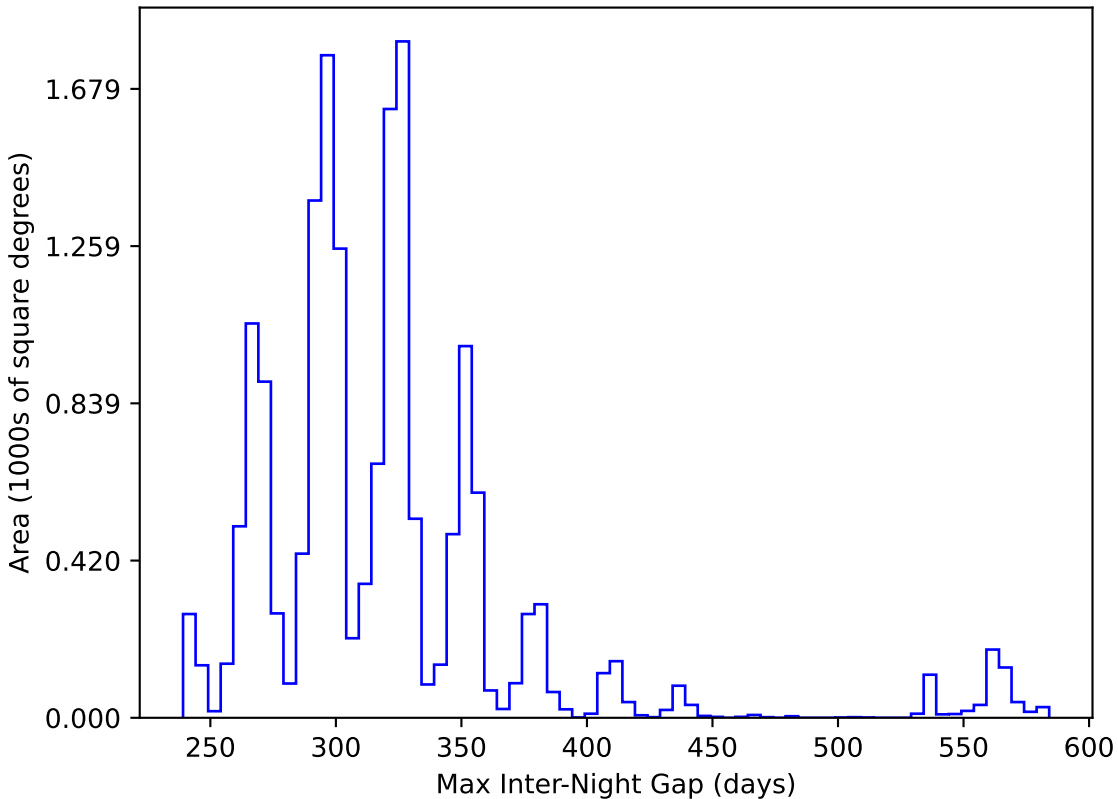
start_date_do180v3.4_10yrs WFD y band: Max Inter-Night Gap
