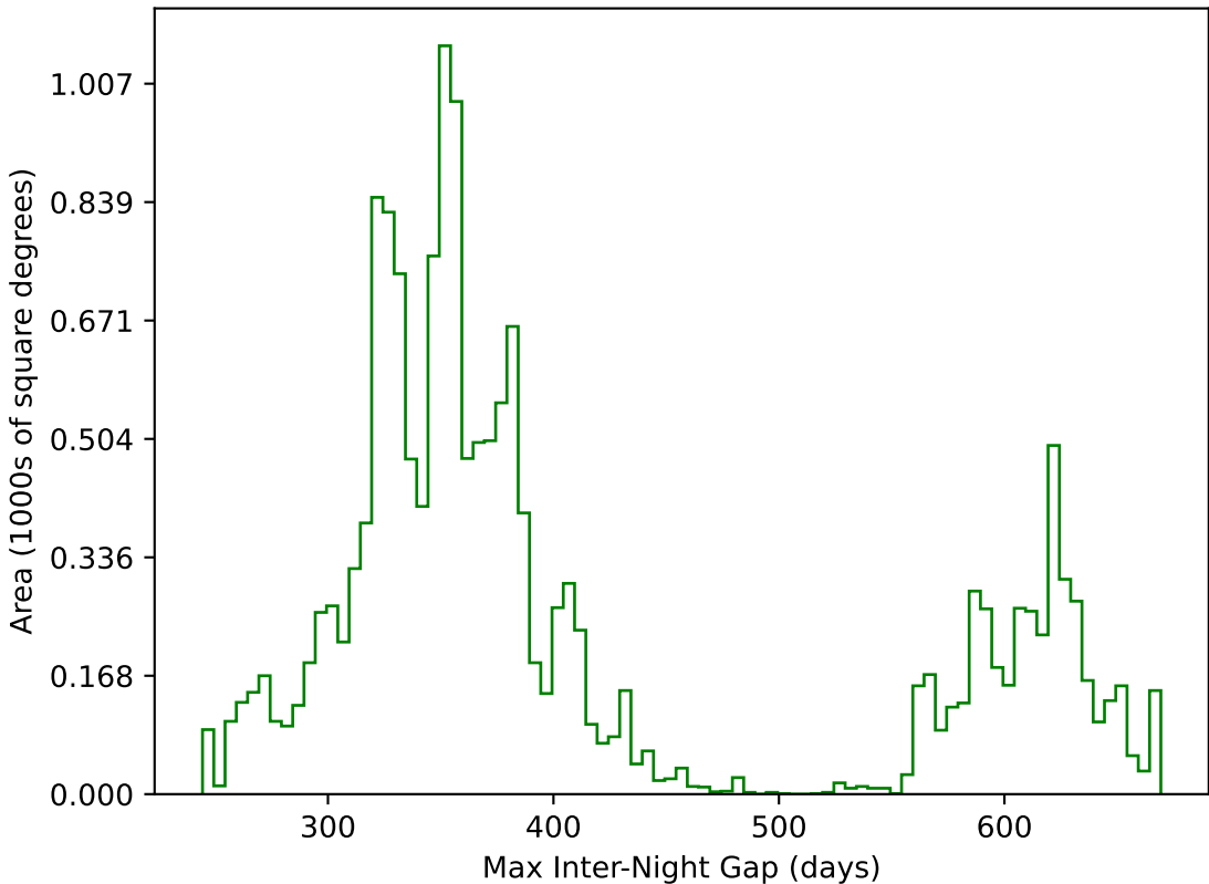
start_date_do180v3.4_10yrs WFD g band: Max Inter-Night Gap
